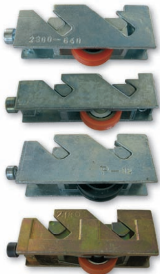
Ruedas Regulables Zamak Zamak Adjustable Rollers for Sliding Windows
