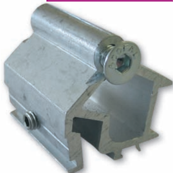
Unión Camara Nacional (40x20) Opened T-Union for Spanish Groove
